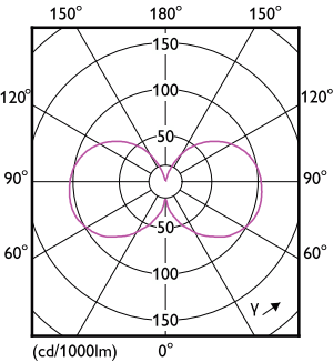
Light Distribution Diagram - MAS LEDCandleDT3.4-40W B22 927 B35CL G
