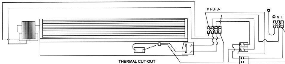
Fig 3 WIRING DIAGRAM - HE7402-31
