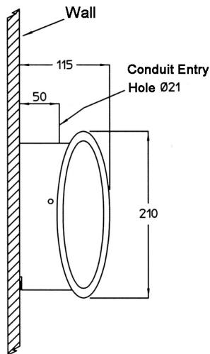
Fig 1 - OUTLINE DRAWING
