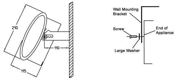
Fig 2 WALL BRACKET ASSEMBLY
