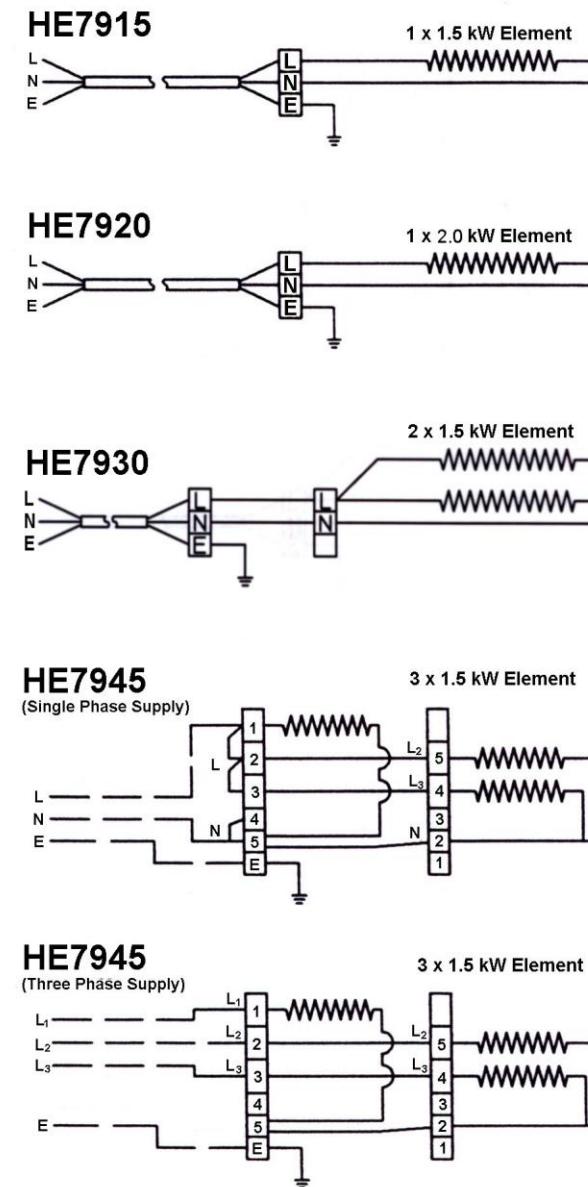
Fig 4 – Circuit Diagrams of Quartz Heaters
