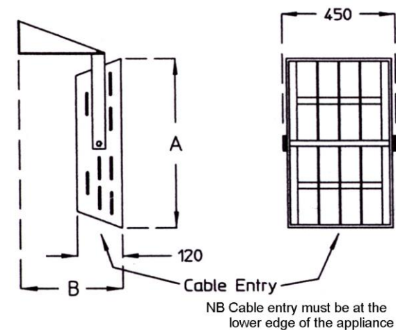
Figure 1 – Outline Dimensions of Quartz Heaters
