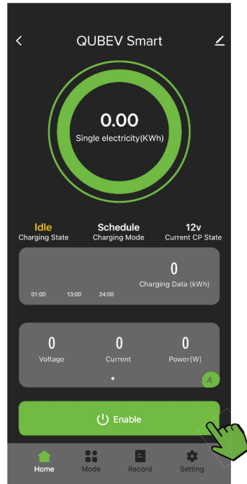
Figure 19 Home Screen
