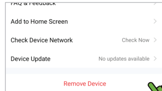
Figure 25 Remove Device
